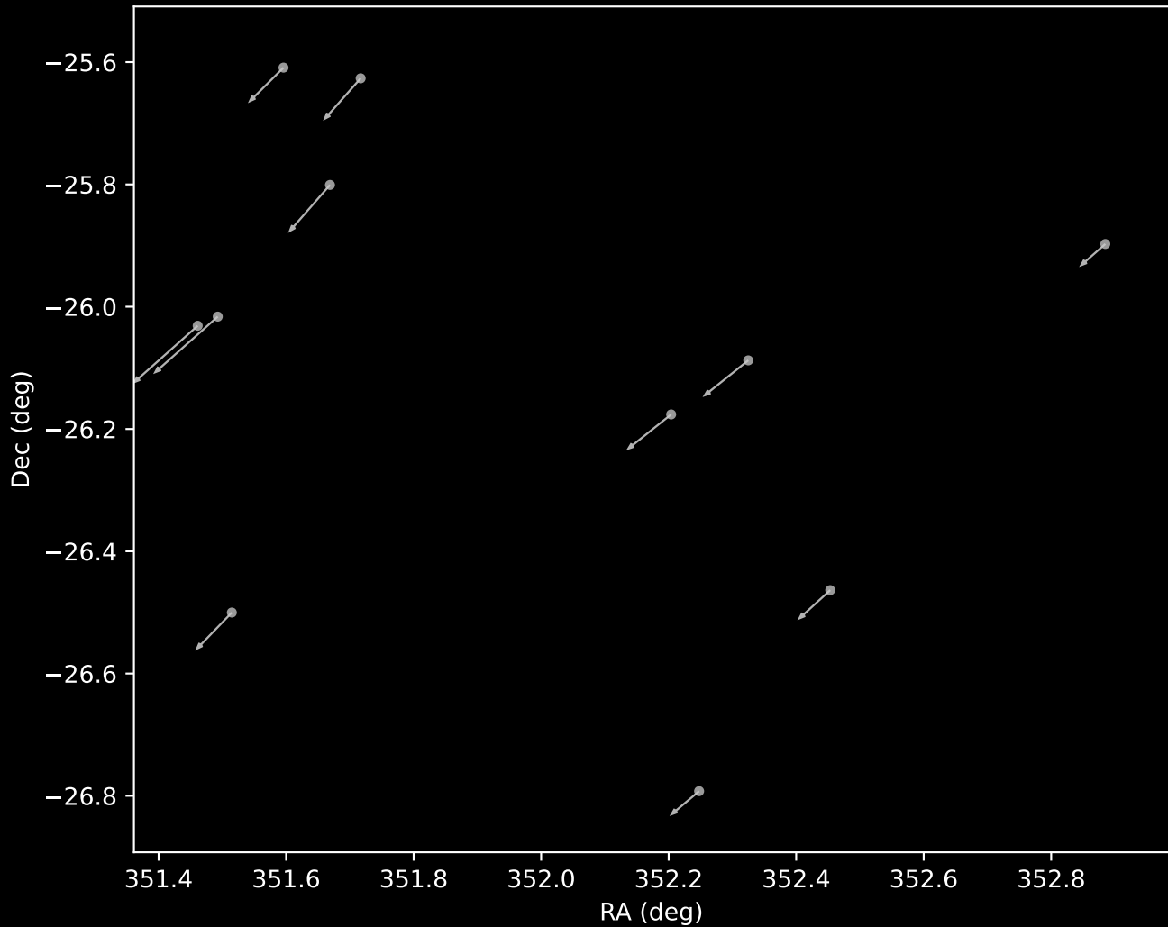
APOGEE DR17 Cluster 15 Proper Motion Vectors (n=11)
