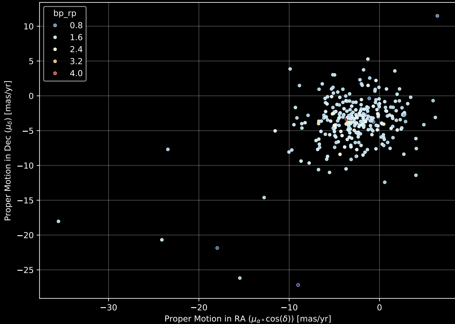
APOGEE DR17 Field: [355+12] Proper Motion Diagram (n= 283)
