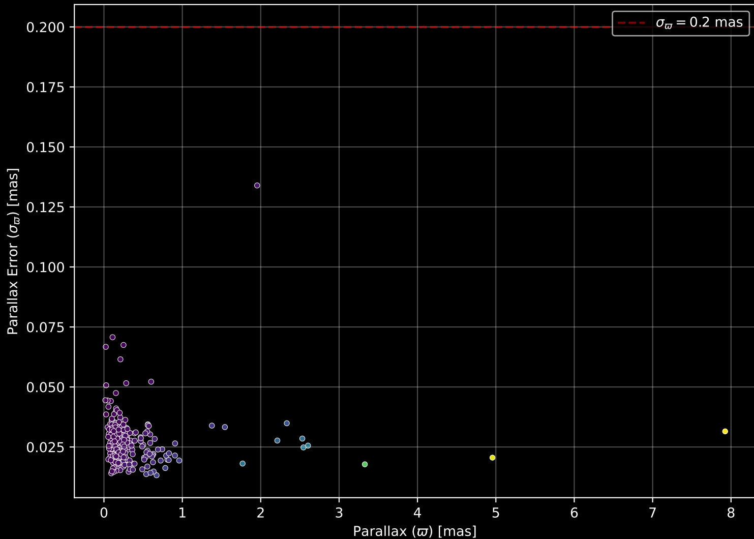
APOGEE DR17 Field: [355+12] Parallax Quality (n= 283)
