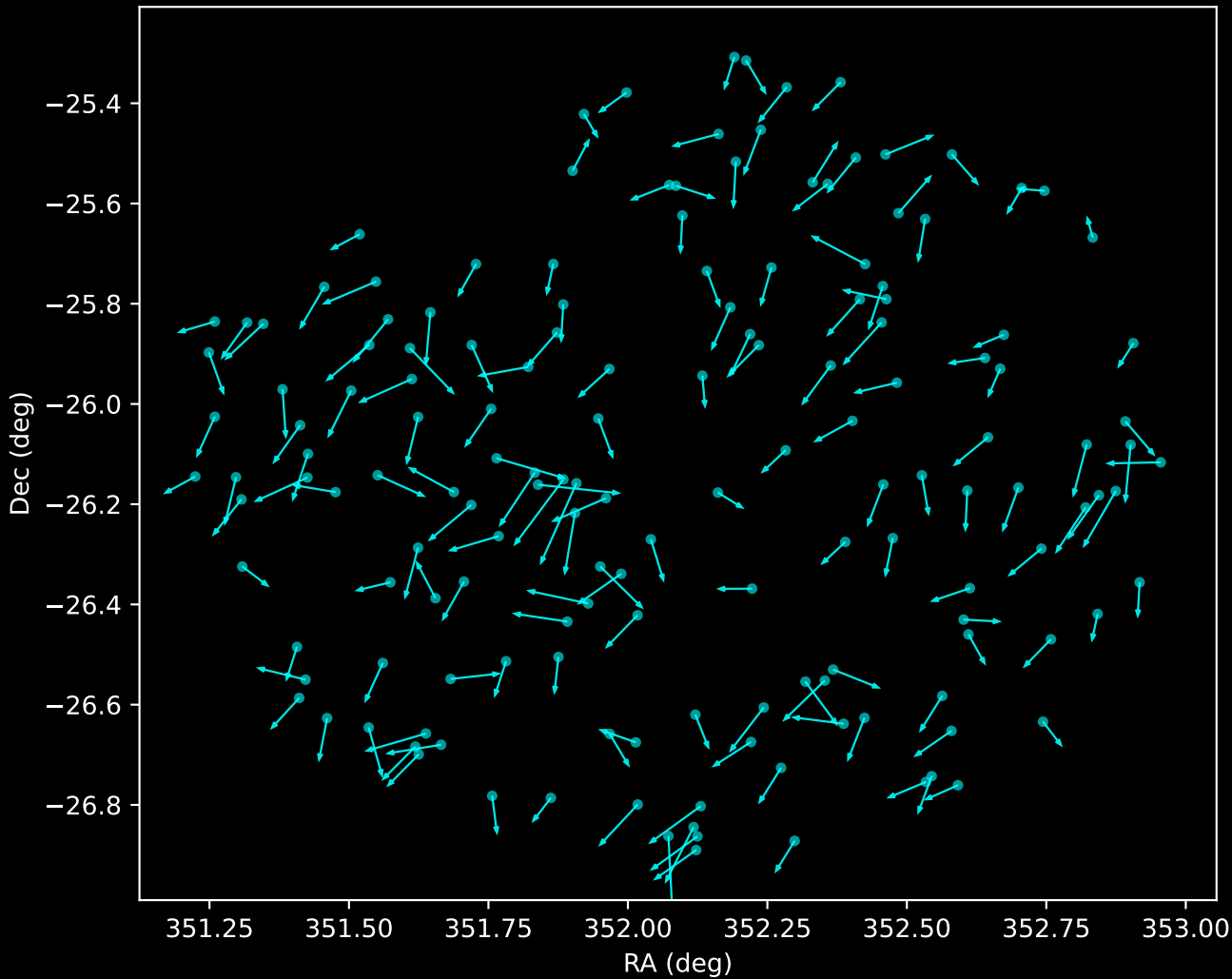
APOGEE DR17 Noise Stream Proper Motion Vectors (n=158)
