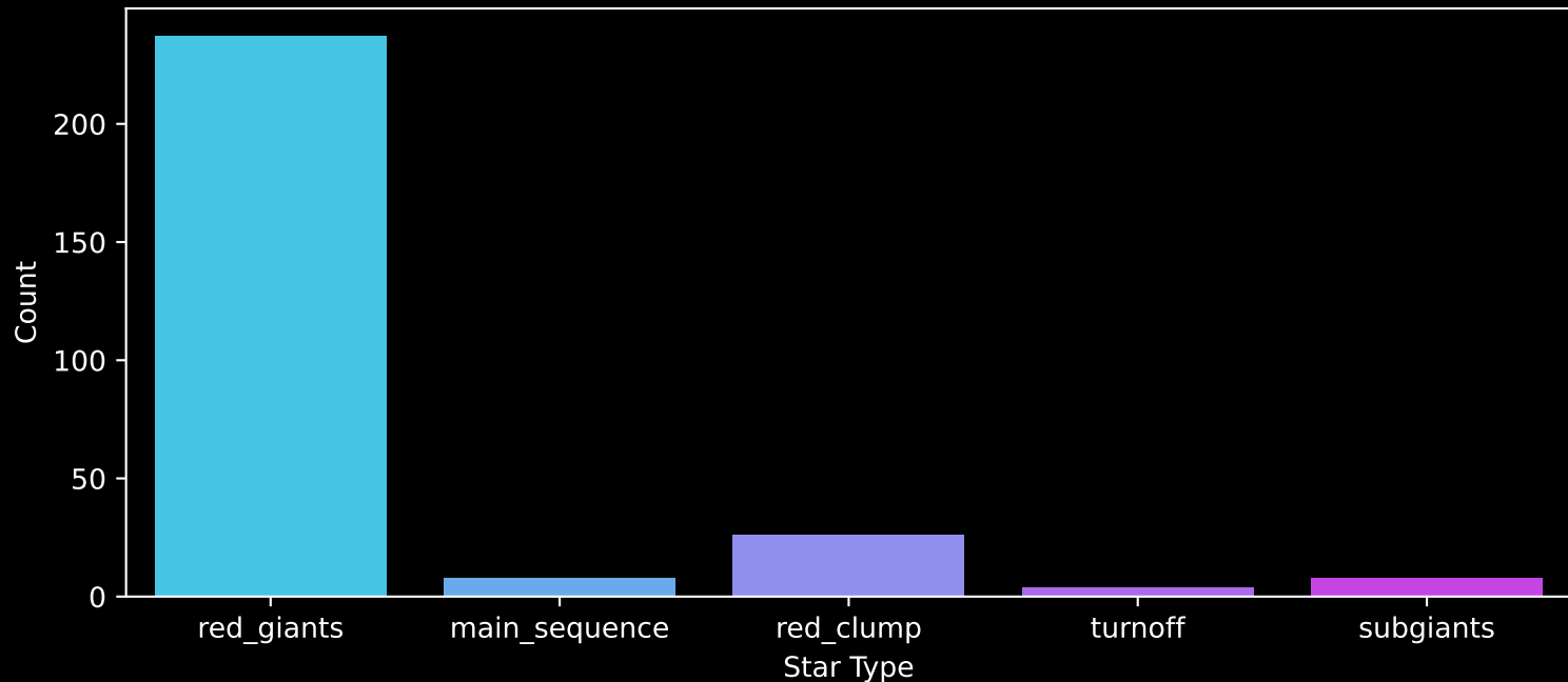
APOGEE DR17 Field: [355+12] Count plot of Star Type
