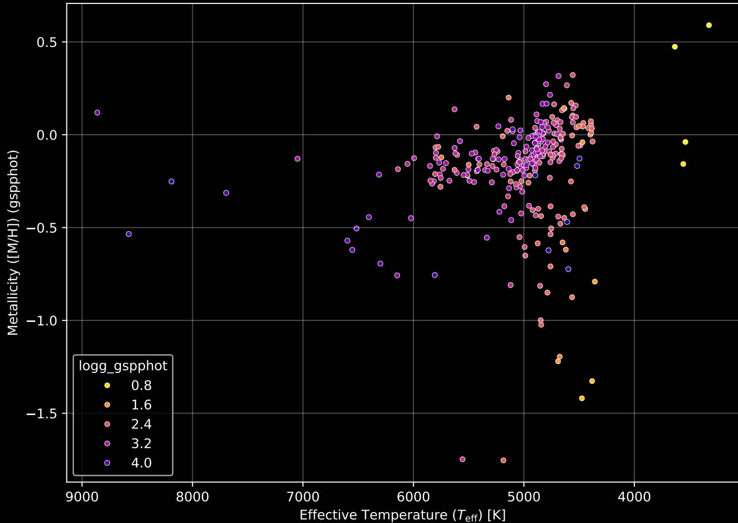
APOGEE DR17 Field: [355+12] Stellar Population Parameters (n= 283)
