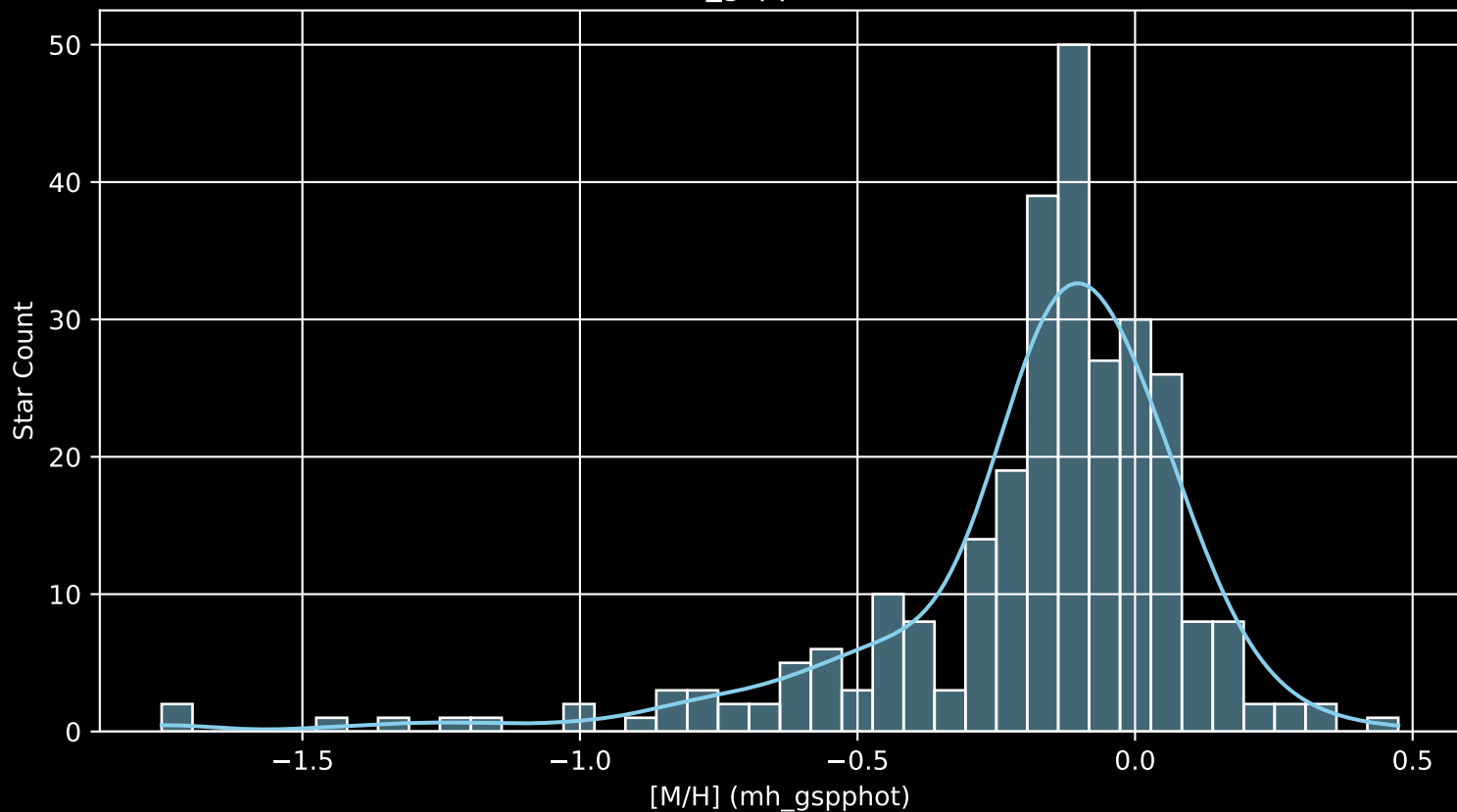
APOGEE DR17 Field: [355+12 [M/H] (mh_gspphot) (n= 282)
